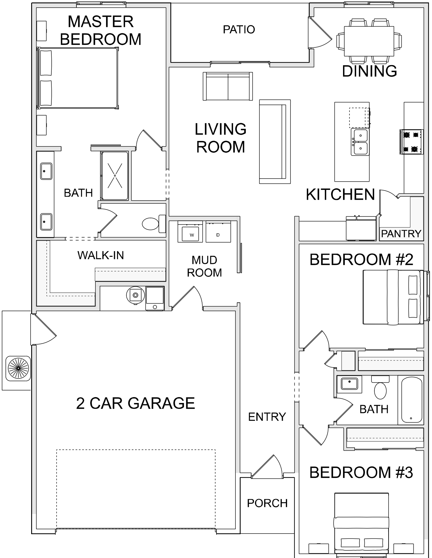
MAIN LEVEL FLOOR PLAN
