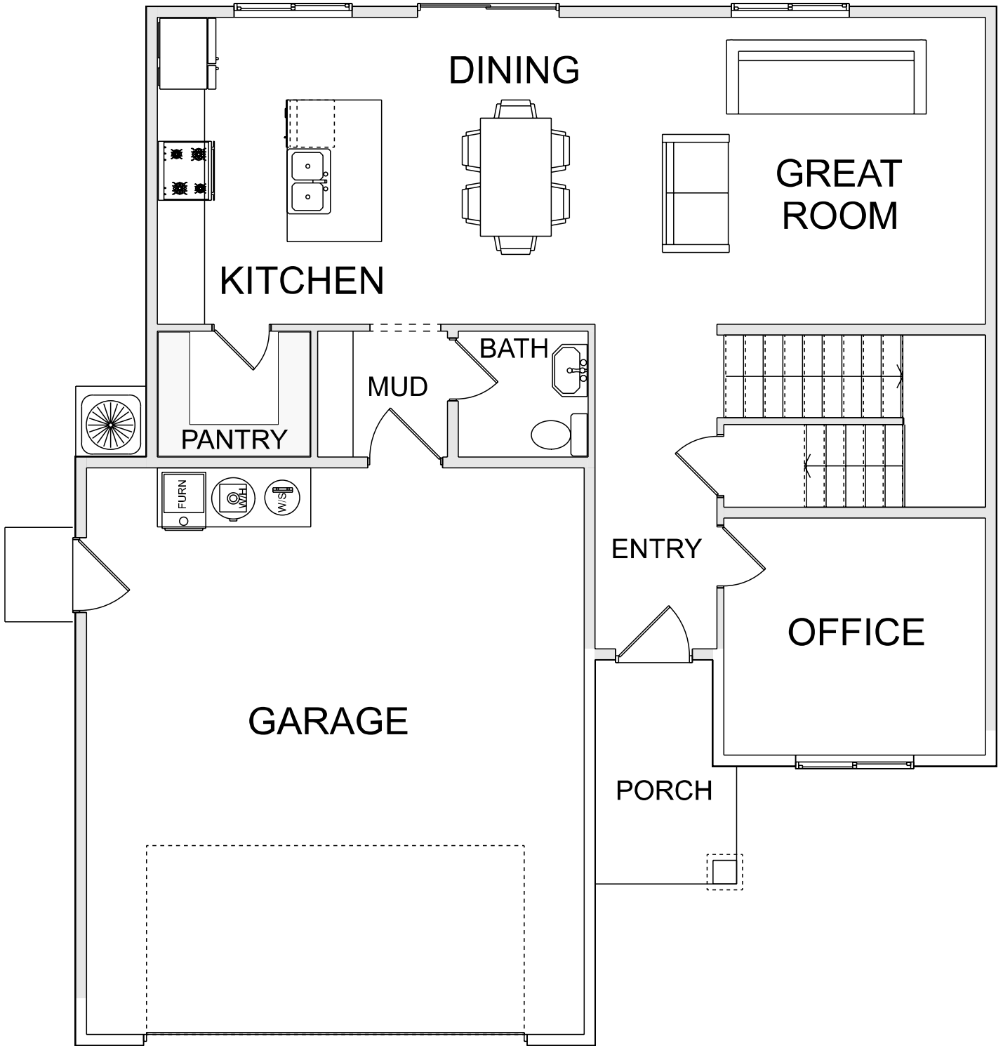
MAIN LEVEL FLOOR PLAN
